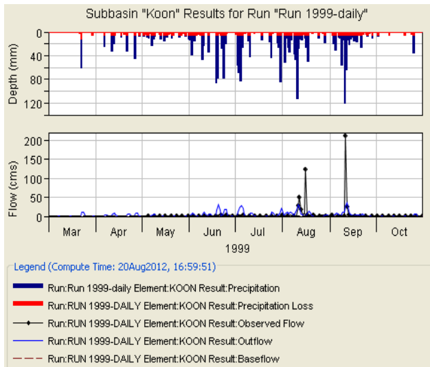
Fig. 6 Observed rainfalls, river flow and simulated flow of Koon
