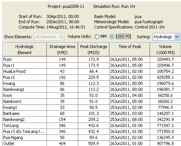
Fig. 8 HMS's simulation result using 1-hr time step in 2011
