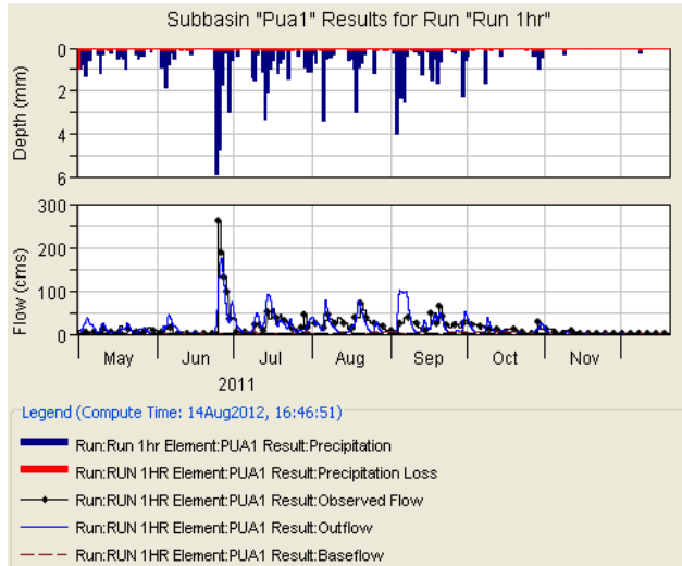
Fig. 7 Observed and simulated results using 1-hr time step in 2011
