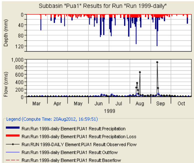
Fig. 5 Observed rainfalls, river flow and simulated flow of Pua1
