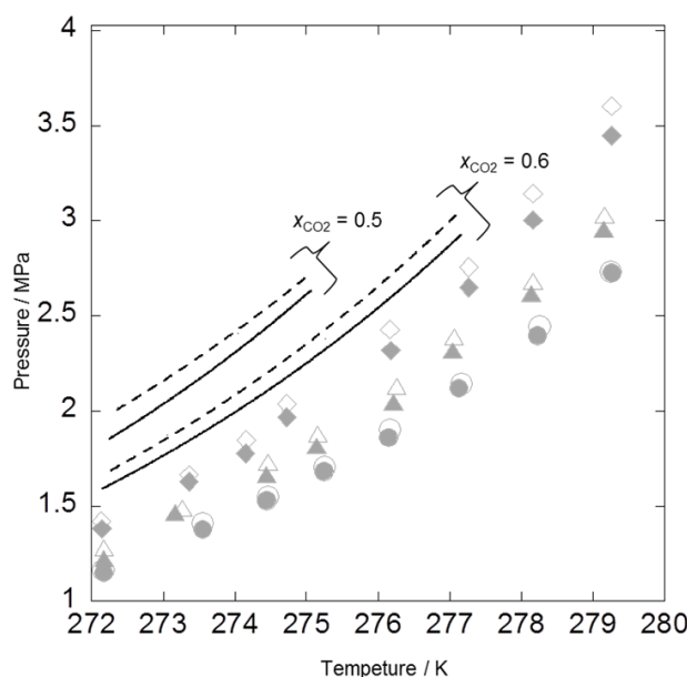
Fig. 3 Three-phase equilibrium p – T data for O_3 + O_2 + CO_2 + H_2O system (solid line, ●, ▲, ◆) and O_2 + CO_2 + H_2O system (dotted line, ○, △, ◇). The data points relevant to the five different levels of x_{CO_2} , the CO_2 mole fraction in the gas phase, are discriminated by their geometries as follows: circles (●, ○) for x_{CO_2} \approx 0.9 ; triangles (▲, △) for x_{CO_2} \approx 0.8 ; rhombuses (◆, ◇) for x_{CO_2} \approx 0.7 ; and (the upper line) for x_{CO_2} \approx 0.6 ; (the lower line) for x_{CO_2} \approx 0.5 . The data for x_{CO_2} \approx 0.6 and x_{CO_2} \approx 0.5 were newly obtained in this study. Other data were obtained in our previous study [6]
