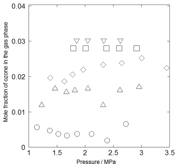
Fig. 4 Three-phase equilibrium pressure versus mole fraction of ozone in the gas phase for O_3 + O_2 + CO_2 + H_2O system ( \circ , \Delta , \diamond , \square , \nabla ). The data points relevant to the five different levels of x_{CO_2} , the CO_2 mole fraction in the gas phase, are discriminated by their geometries as follows: circle ( \circ ) for x_{CO_2} \approx 0.9 ; triangle ( \Delta ) for x_{CO_2} \approx 0.8 ; rhombuse ( \diamond ) for x_{CO_2} \approx 0.7 ; and square ( \square ) for x_{CO_2} \approx 0.6 ; triangle ( \nabla ) for x_{CO_2} \approx 0.5 . The data for x_{CO_2} \approx 0.6 and x_{CO_2} \approx 0.5 were newly obtained in this study. Other data were obtained in our previous study [6]
