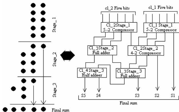
Fig. 8 Bit reduction technique using conventional compressors
