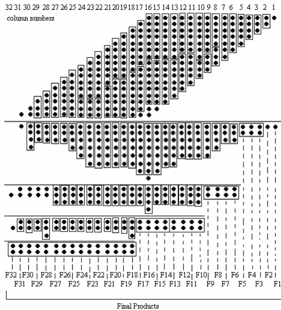
Fig. 7 Architecture of 16x16 bit multiplier
