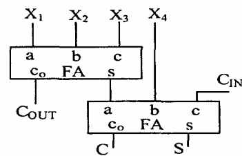
Fig. 1 Conventional 4-2 compressor
