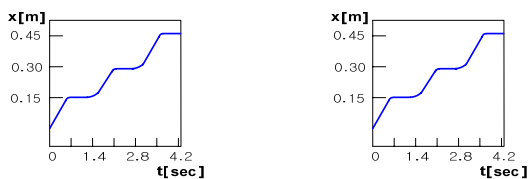
(a) ZMP trajectory in sagittal plane (b) ZMP trajectory in lateral plane
