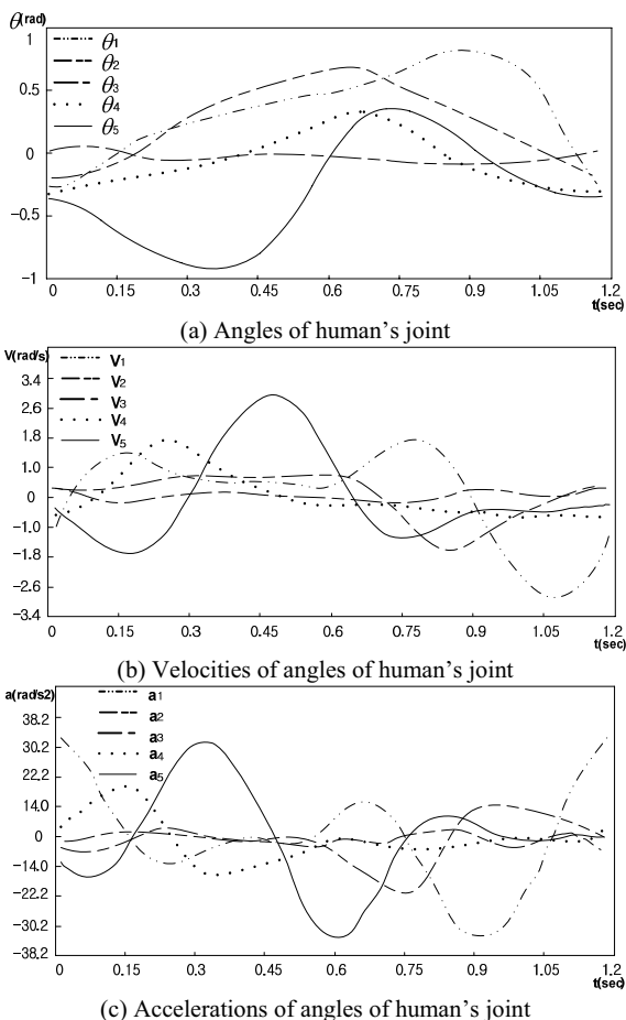
Fig. 9(a) is shows joint's the angles by using the joint's pose
