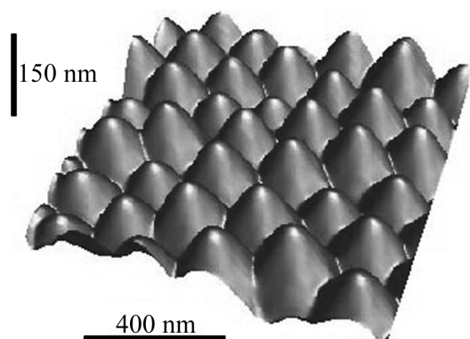
Fig. 4 Atomic Force Microscope generated 3D image of a cicada wing array
