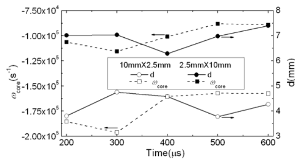
Fig. 4 The vorticity at the center of the core and the distance between the two vortex cores of these two simulations
