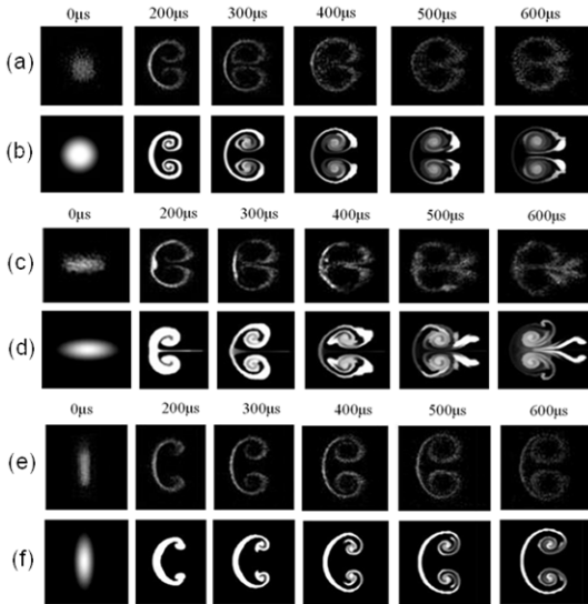
Fig. 1 Multiple dynamics images and numerical simulation results by MVFT at t=200, 300, 400, 500, \text{ and } 600 \mu\text{s} after shock passage. [The experiments corresponding (a), (c), and (e), and the simulations corresponding (b), (d), and (f)]
