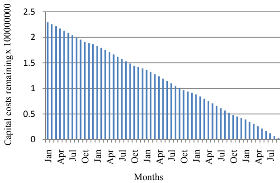
Fig. 3 System construction payback period for tracking system
