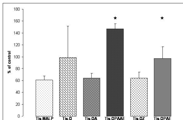
Fig. 2 Expression of \alpha_3\beta_1 integrin after 24 hrs
