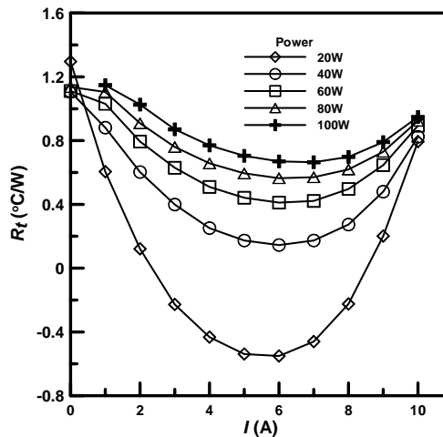
Fig. 8 overall resistance under every heating power and input current, R_T increases with heat load. Due to the contrary trends of R_{TEC} and R_{HS} for input current, an optimal input current exists in R_T
