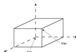
Fig. 1 Hyperbox in R^3 defined from its min and max points
