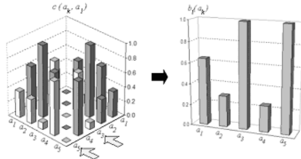
Fig. 6 The symmetric distance function between categories c(a_k, a_l) and the membership function b_j(a_k) of the hyperbox defined by categories e_j = a_3 and f_j = a_5
