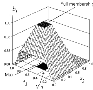
Fig. 3 Membership function of the hyperbox in I^2 defined by the minimum v_j = (0.4, 0.2) , the maximum w_j = (0.6, 0.4) and the parameter \gamma = 3
