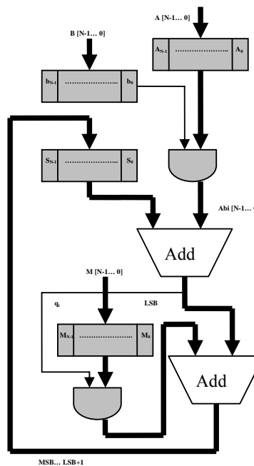
Fig. 4 Montgomery multiplier architecture based on algorithm (2)
