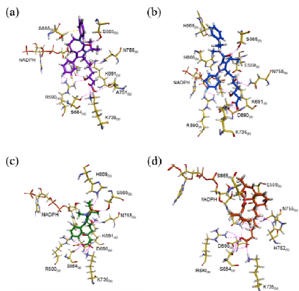
Fig. 4 Binding mode of four HMGR inhibitors at the active site. (a) INH1, (b) INH2, (c) INH3, and (d) INH4 were shown as as purple, blue, green, and orange stick model and active site residues were drawn as yellow stick model. Dash lines indicate hydrogen bond (magenta) and hydrophobic interaction (yellow), respectively
