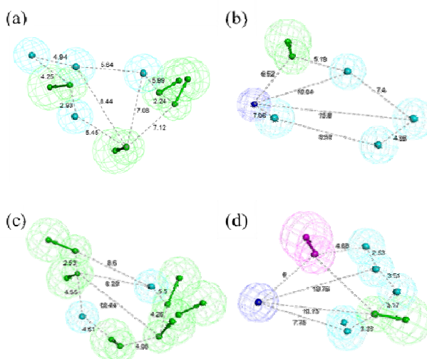
Fig. 5 Structure-based pharmacophore models of each complex. (a) Pharm 1, (b) Pharm2, (c) Pharm3, and (d) Pharm 4. HBA, HBD, HYP, and NI features were represented in green, magenta, cyan, and blue color, respectively
