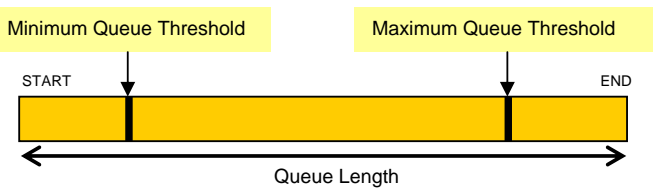
Fig. 3 Representation of a Hybrid Sender-Receiver Node's Queue
