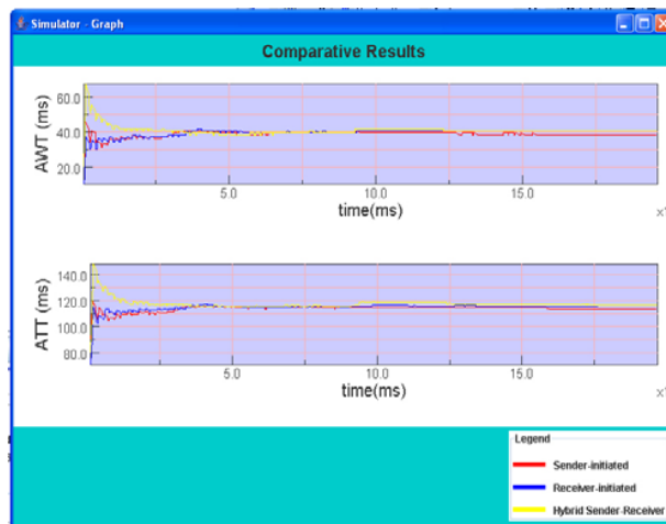
Fig. 9 Graphs for Comparative Simulation in 10 Nodes Environment
