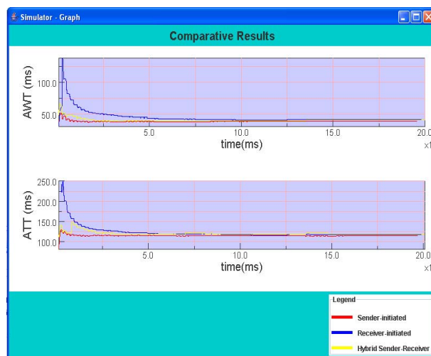
Fig. 10 Graphs for Comparative Simulation in 50 Nodes Environment
