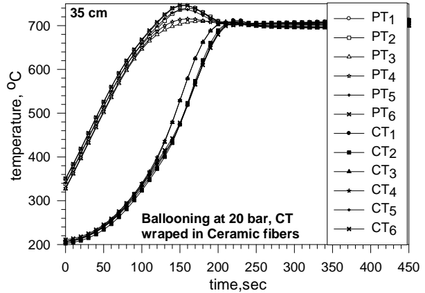
Fig. 7(c) Temperature variation of the PT-CT with time at 35 cm from rectifier end
