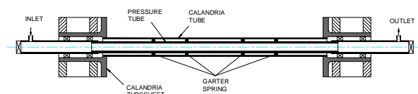
Fig. 1 Schematic of Indian PHWR Reactor Channel
