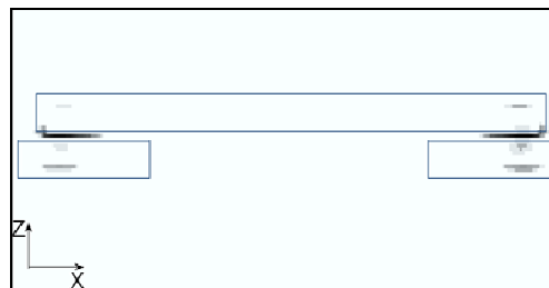
Fig. 6 Field profile showing the localization of the field in the \text{SiO}_2 material in the overlap of the two disks of the structure studied. The frequency of the pulse is 276\text{THz} and the thickness of the two layers is 0.12\mu\text{m}
