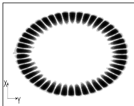
Fig. 5 WGM created in the \text{SiO}_2 material in the overlap of the two disks of the structure studied. The frequency of the pulse is 276\text{THz} and the thickness of the two layers is 0.12\mu\text{m}
