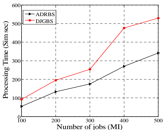
Fig. 5 Job processing time
