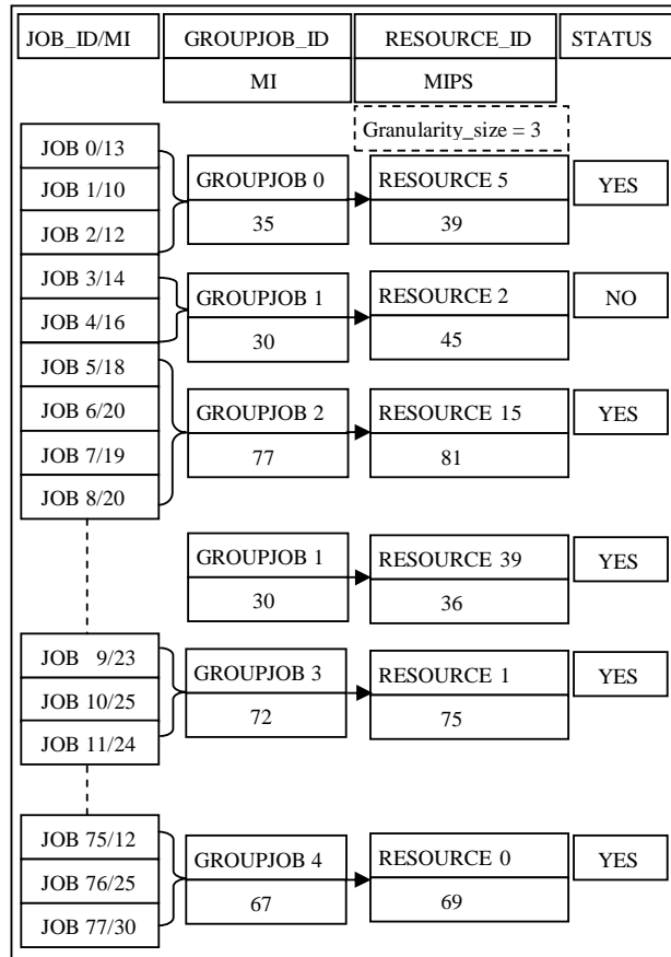
Fig. 4 Example of the proposed job scheduling strategy
