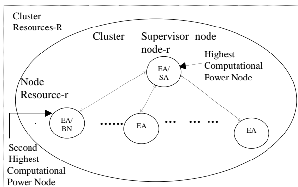
Fig. 2 Supervisor node selection
