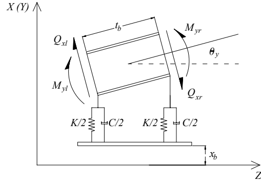
Fig. 4 Bearing model
