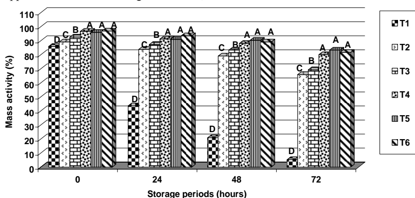
T1 = fresh semen, T2 = semen diluted with AD2D alone, T3 – T6 = semen samples diluted with AD2D supplemented with 2 ml, 4 ml, 6 ml or 8 ml of olive oil / 100 ml of diluent, respectively. AD2D = Al – Daraji 2 diluent. Bars with different superscripts differ significantly (p < 0.05). Each value represented the mean of 20 measures that conducted during 10 consecutive weeks.
