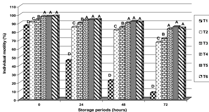
T1 = fresh semen, T2 = semen diluted with AD2D alone, T3- T6 = semen samples diluted with AD2D supplemented with 2 ml, 4 ml, 6 ml or 8 ml olive oil / 100 ml of diluent, respectively. AD2D = Al – Daraji 2 diluent. Bars with different superscripts differ significantly (p < 0.05). Each value represented the mean of 20 measures that conducted during 20 consecutive weeks.
