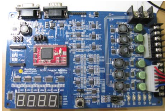
Fig. 9 Control Board
