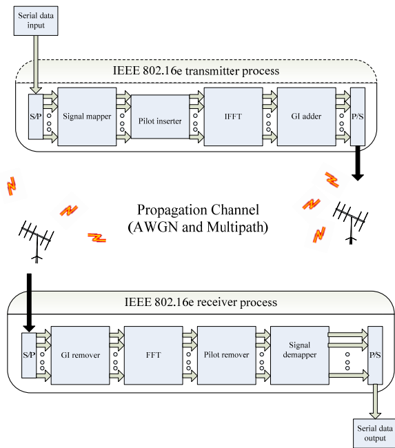
Fig. 2 The flowchart of the OFDM system
