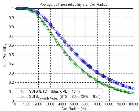
Fig. 5 The coverage with and without Rayleigh fading over the SUI-6 channel
