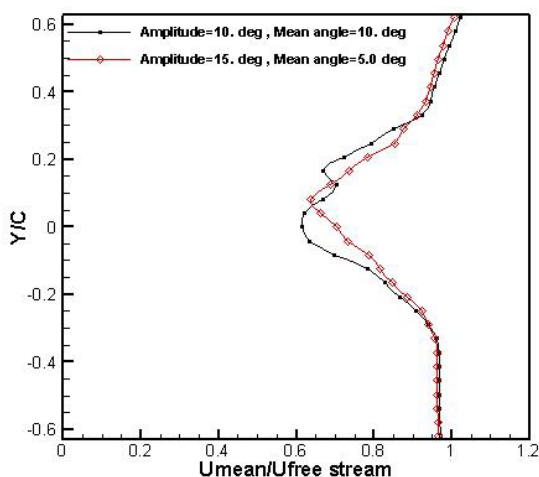
Fig. 13 Mean velocity profiles ( A = 10^\circ, \alpha_0 = 10^\circ and A = 15^\circ, \alpha_0 = 5^\circ )
