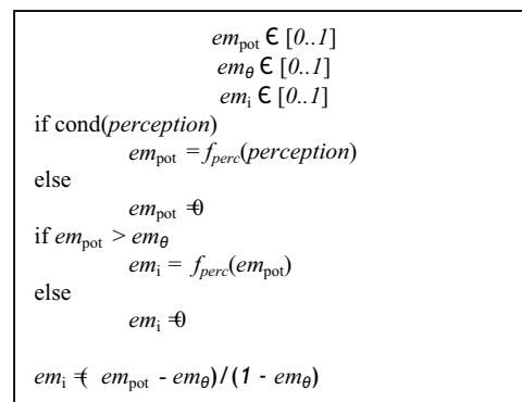
Figure 2. Computation of an emotion [7] 2
