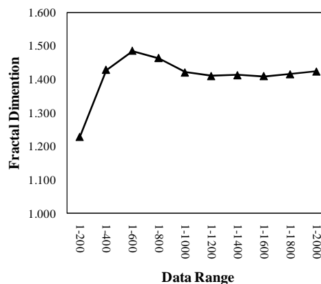
Fig. 5 Fractal dimension of Ghareh-Aghaj River weekly time series in different selection windows by R/S Method
