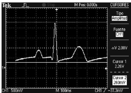
Fig. 12 ECG Acquired Signal after the DC Level Adjustment
