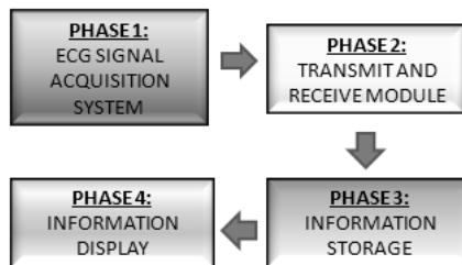
Fig. 4 Methodology
