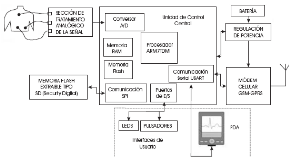
Fig. 2 CARE Monitoring device [5]
