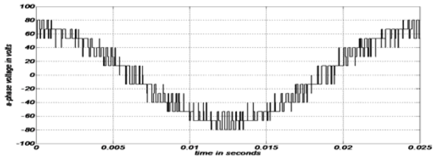
Fig. 8.b A-phase phase voltage with f_1=40\text{Hz} .
