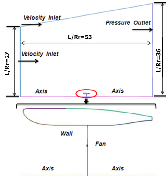
Fig. 3 Computational field and boundary condition settings
