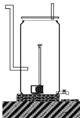
Fig. 5 Installation of a smoke and smell filter case
