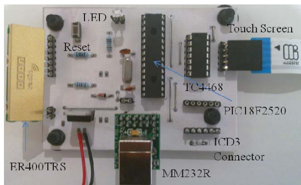
Fig. 4 Top view of the completed soldered PCB
