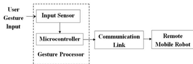
Fig. 3 System block diagram
