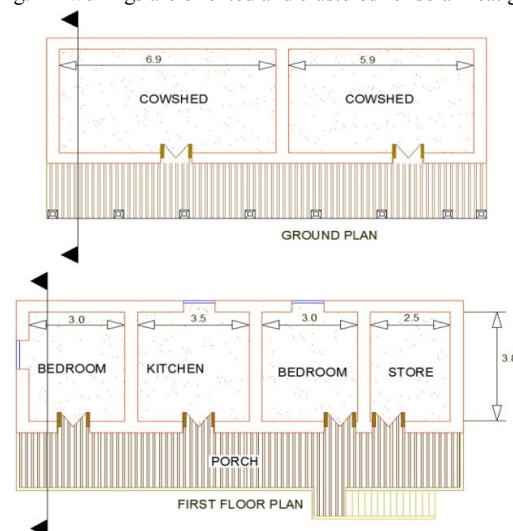
Fig. 3 Typical floor plans of dwellings
