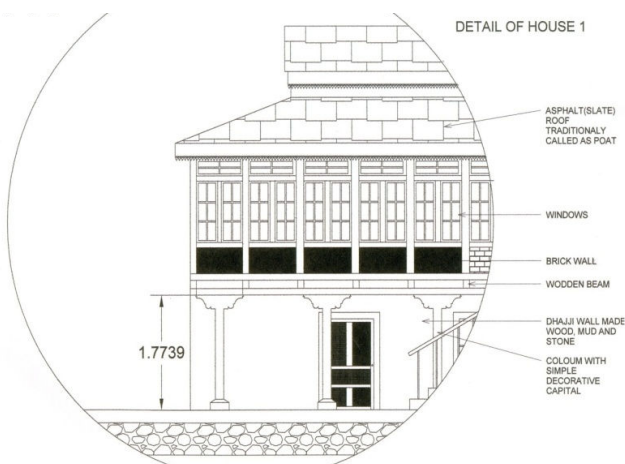
Fig. 9 Featured architectural elements of the dwellings
