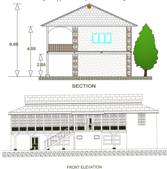
Fig. 4 Typical section & elevation of dwelling
