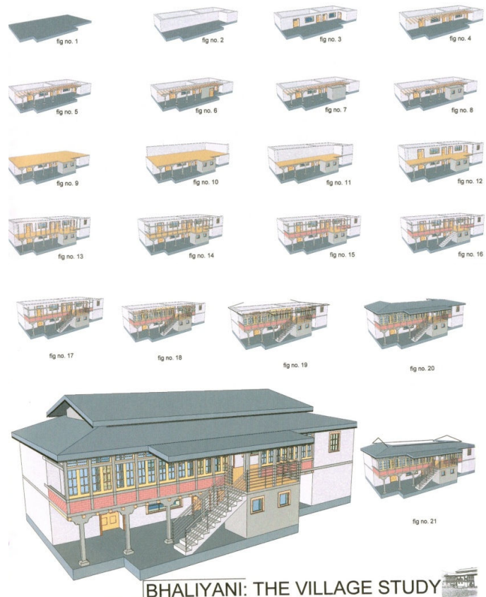
Fig. 10 Construction process of the dwellings in the settlement
