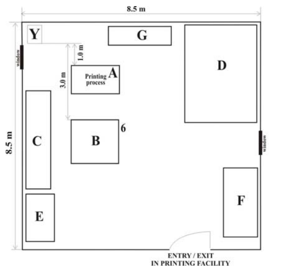
A - desk for manual screen printing process B, C - desk for drying of printed sheets (products) D - rotary die-cutter machine E - wash sink for screen F - mounting table and desk for screen exposure G - shelf for raw printing materials (inks, ink reducers, etc.) Y - air sampler (placed on the floor)
