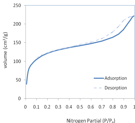
Fig. 1 Nitrogen adsorption-desorption isotherm for calcined HMS
