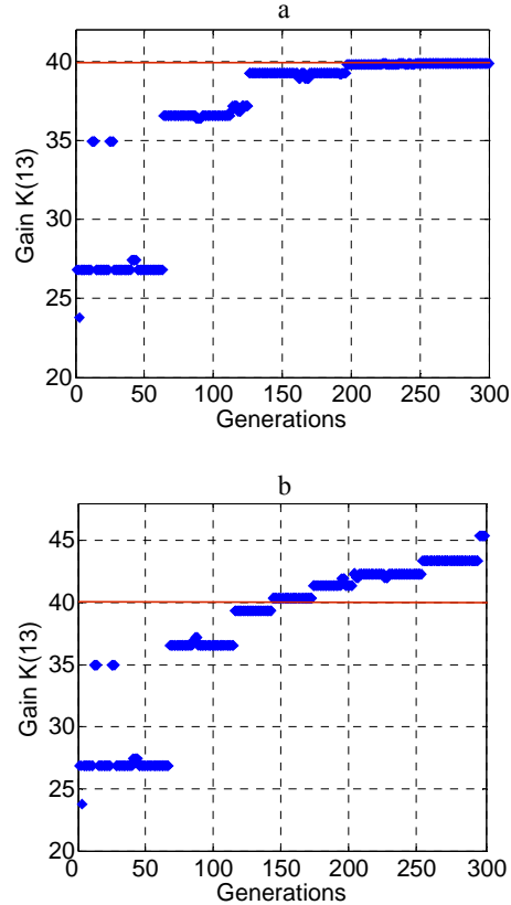
Fig. 6 Optimization evolution of the PSS parameter ( K_{(13)} ): a: using fixed search space boundaries b: using dynamic search space boundaries
