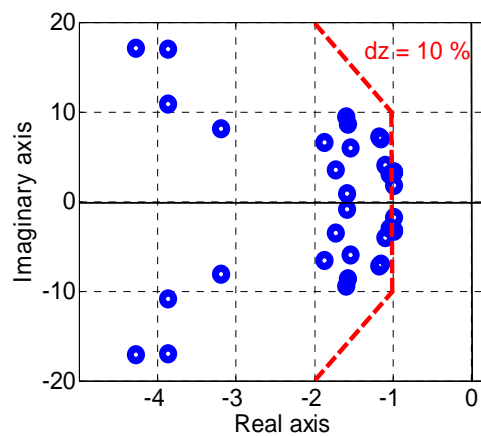
Fig. 4 Electromechanical modes of closed-loop system
