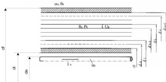
Fig. 6 Bushing calculation model
