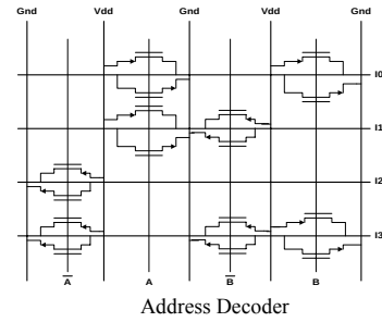
Address Decoder
