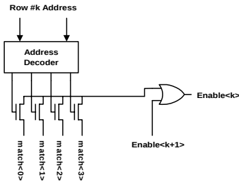
Fig. 5 A sample 2-bit Pseudo-nMOS comparator
