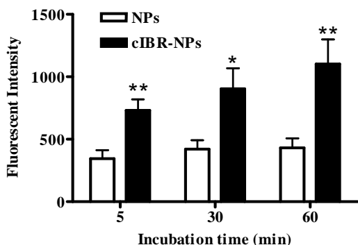
Fig. 7 The comparison between the binding and internalization of cIBR-NPs and NPs after incubation with Mixed PBMC-Molt-3 cells. Results are given as mean ± S.D. (n=10); * indicates p < 0.05 and ** indicates p < 0.01
