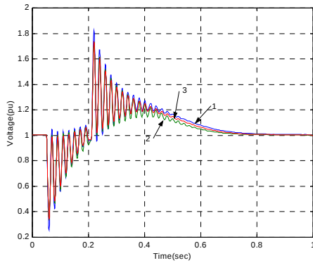
Fig. 3c Terminal voltage, (1) detailed model, (2) singular perturbation model, (3) integral manifolds model
