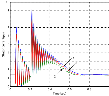
Fig. 3b Induction generator 2 stator current, (1) detailed model, (2) Singular perturbation model, (3) integral manifolds model
