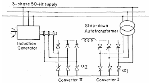
Fig. 2 Schematic representation of DOIG
