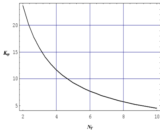
Fig. 2 Optimal radio capacity K_{op} of a single-cell SS MIMO system versus the number of transmit antennas N_T in a Rayleigh fading environment
