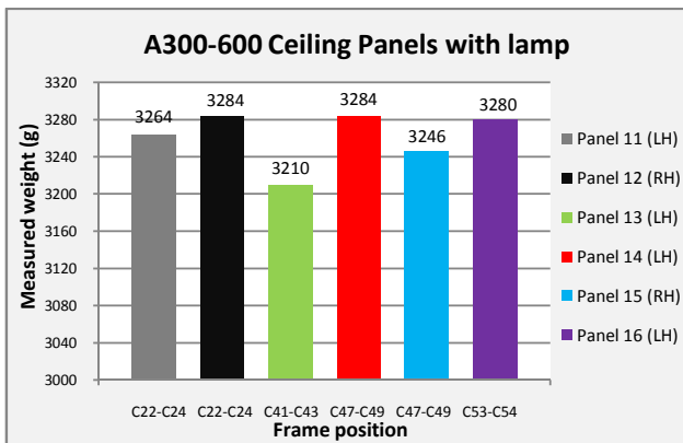
Fig. 9 Measured weight of ceiling panels with lamp
