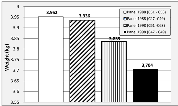
Fig.17: Weight of different real aged ceiling panels
