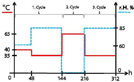
Fig. 13 Climate Cycles for determination of changes in weight and deflection
