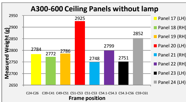
Fig. 10 Measured weight of ceiling panels without lamp
