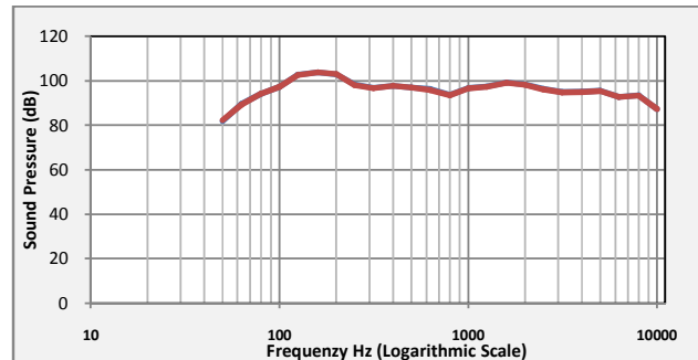
Fig. 6 Sound pressure in reverberation room
