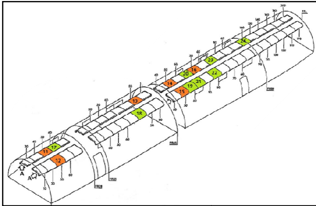
Fig. 8 Position of ceiling panels in the cabin of an Airbus A300-600
