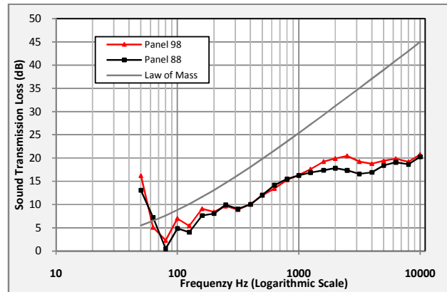
Fig. 19 Transmission Loss of different aged ceiling panels
