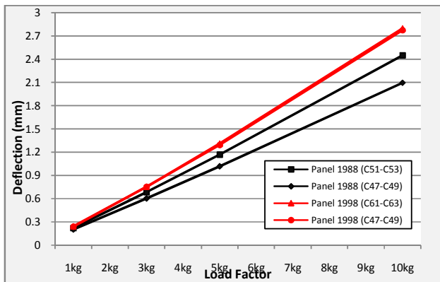
Fig. 18 Deflection of different real aged ceiling panels
