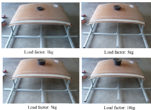
Fig. 5 Sequence of loading the ceiling panels
