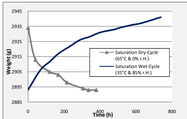
Fig. 11 Absorption and discharge of humidity until saturation
