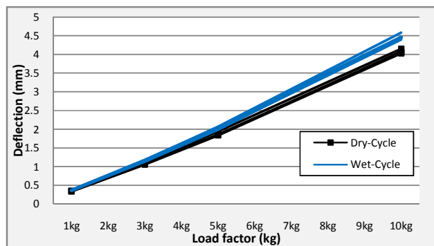
Fig. 12 Deflection of ceiling panel depending on the climate-cycle
