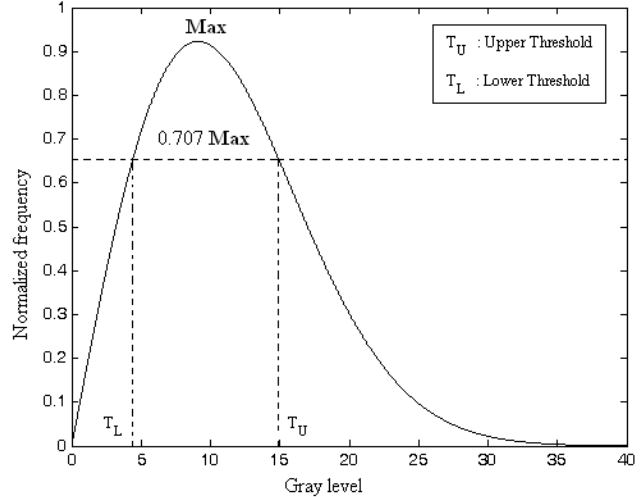
Fig. 1 An example of selecting T_L and T_U .
