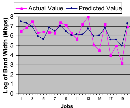
Fig. 8 Actual & Predicted Band width for 20 test cases
