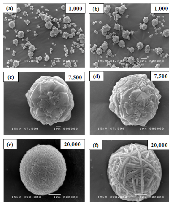
Fig. 2 SEM images of zeolite LSX-A and LSX-B at different magnification
