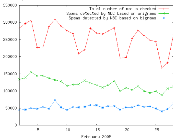
Fig.2 Performance of naïve Bayesian classifiers working at CERN
