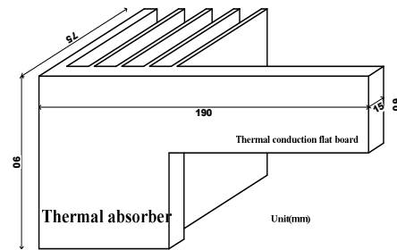
Fig. 6 Thermal absorber and thermal conduction flat board
