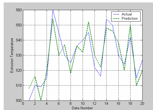
Fig. 8 Graph showing outputs versus targets for extrusion temperature
