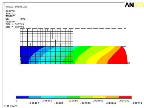
Fig.2 FEM simulation
