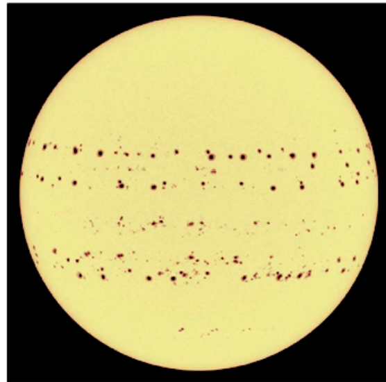
Fig. 5 Sunspot image fusion in July 2001
