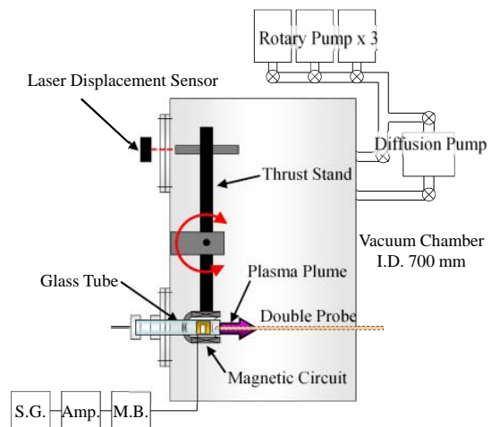
Fig. 2 Schematic of experimental setup
