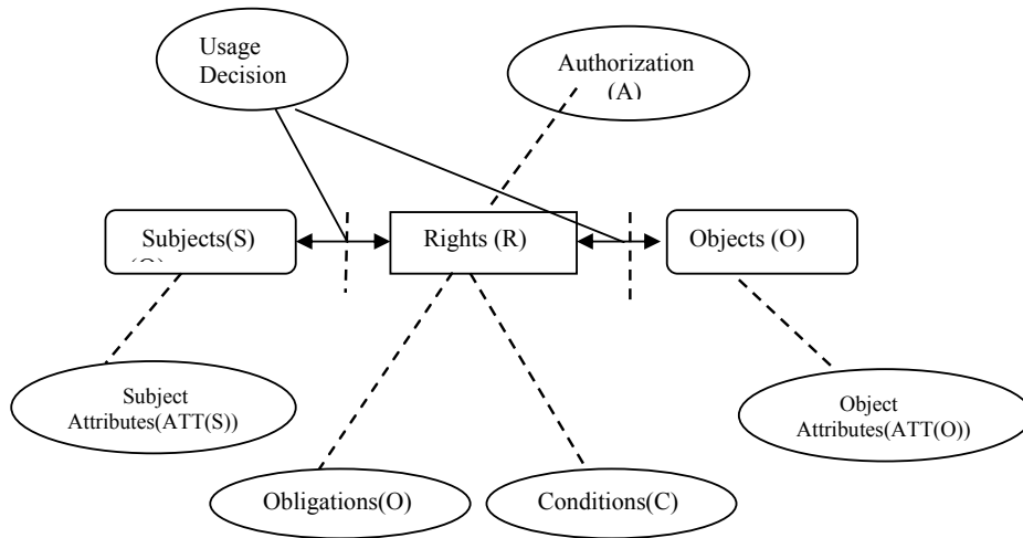
Fig. 2 Components of Usage Control Model
