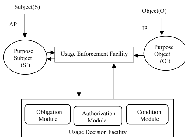
Fig. 3 UAC Architectures on Access Purpose Authorization
