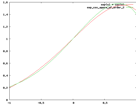
Fig. 6. Approximating \exp(x) * \cos(x) using Chebyshev
