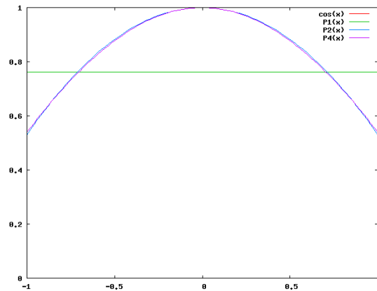
Fig. 1. Approximating \cos(x) using Chebyshev
