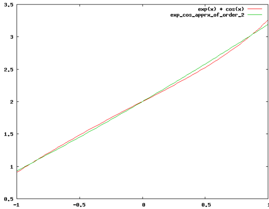
Fig. 4. Approximating \exp(x) + \cos(x) using Chebyshev
