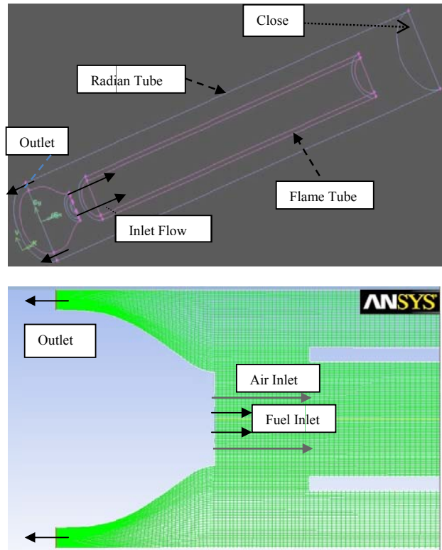
Fig. 1 Configuration of the MILD combustion burner
